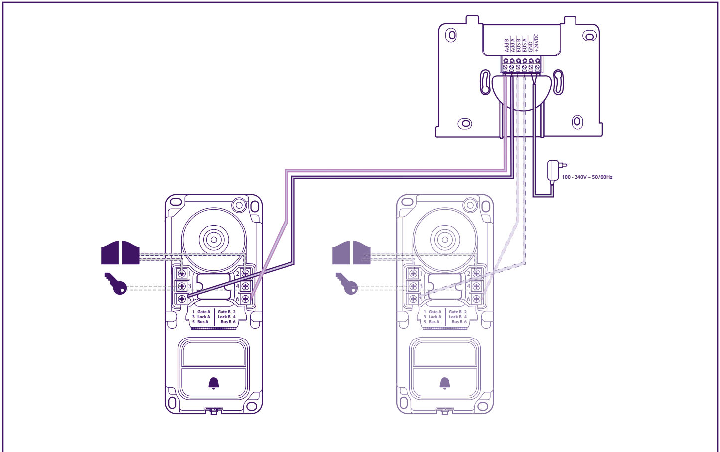
Additional outdoor station Philips Connect 3 / V1
