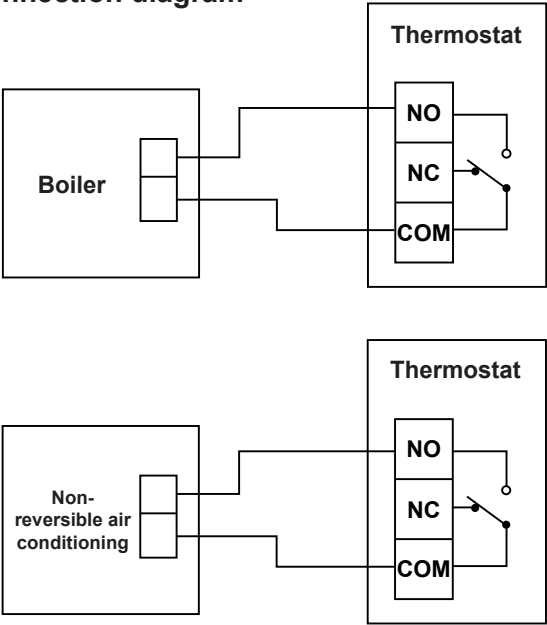
Connection diagram
